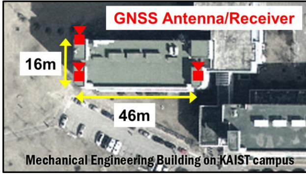
Figure 8. Configuration of LADGNSS Test-bed at KAIST
