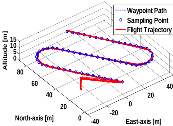
Figure 6. Waypoint Path (Defined Guidance path), Flight Trajectory (Estimated Position) and Sampling Points with Constant Interval
